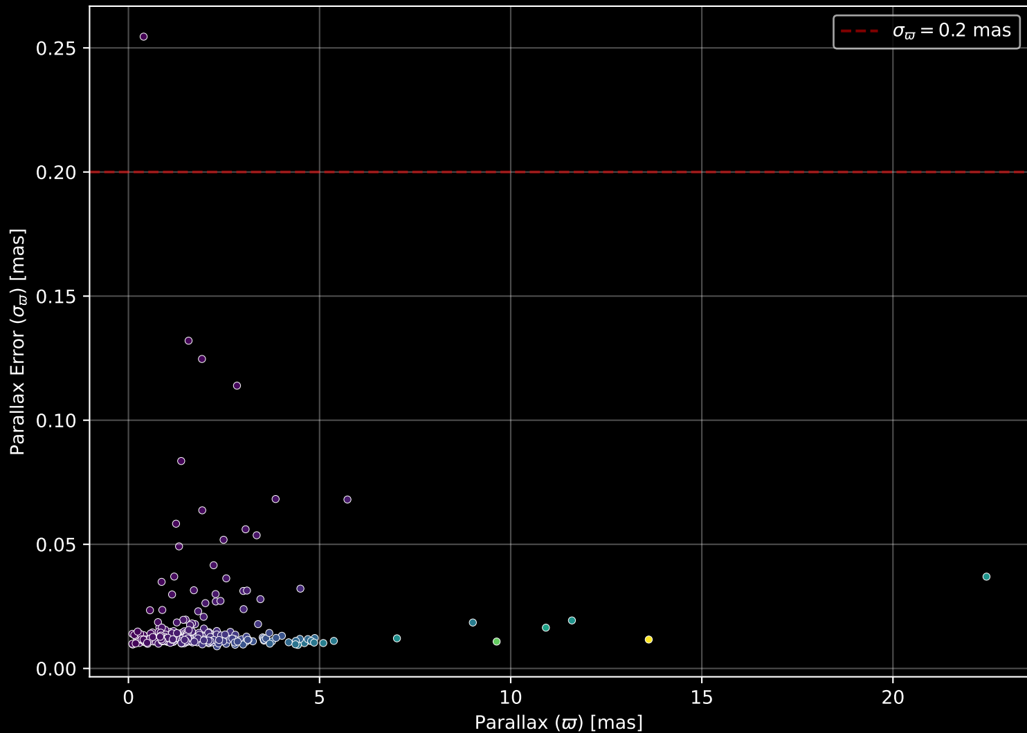
GALAH DR4 Field: [6927] Parallax Quality (n= 298)
