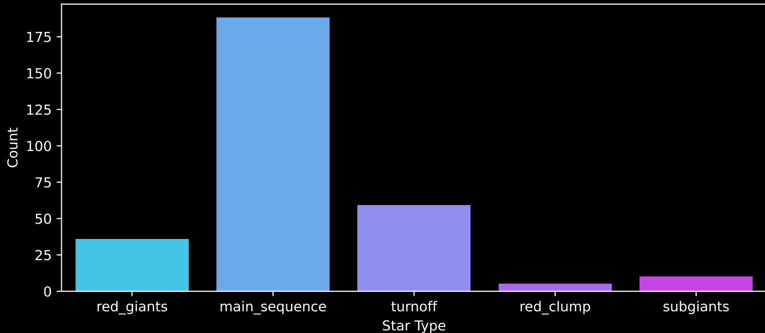
GALAH DR4 Field: [6927] Count plot of Star Type
