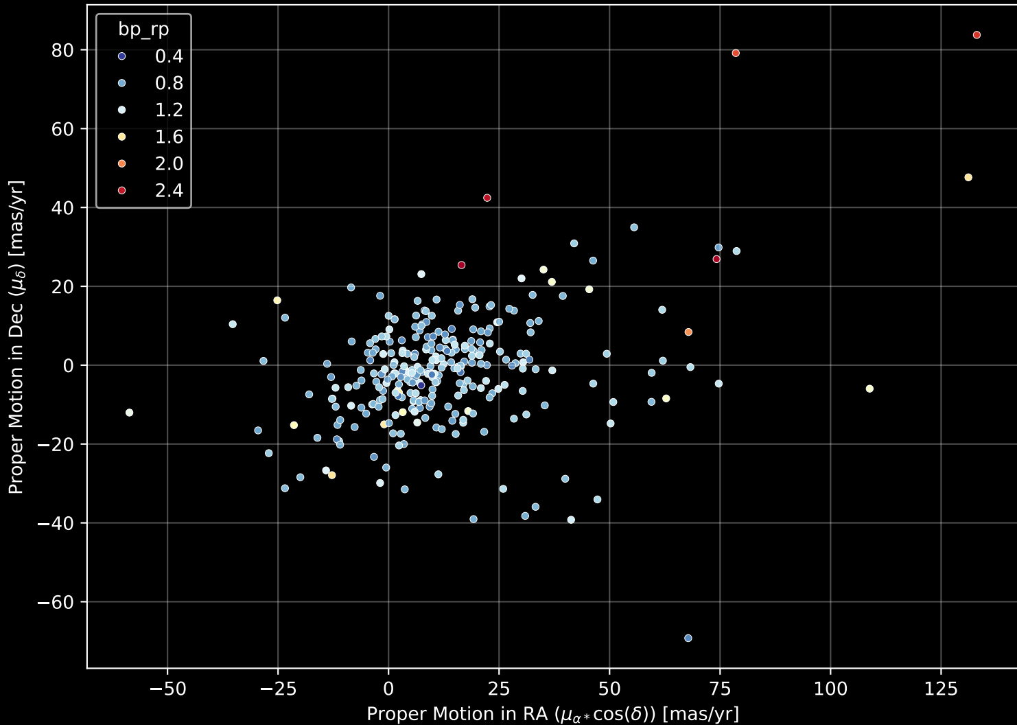
GALAH DR4 Field: [6927] Proper Motion Diagram (n= 298)
