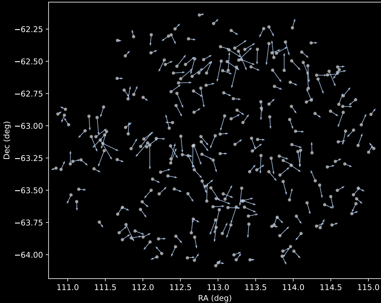
GALAH DR4 Cluster 1 Proper Motion Vectors (n=258)
