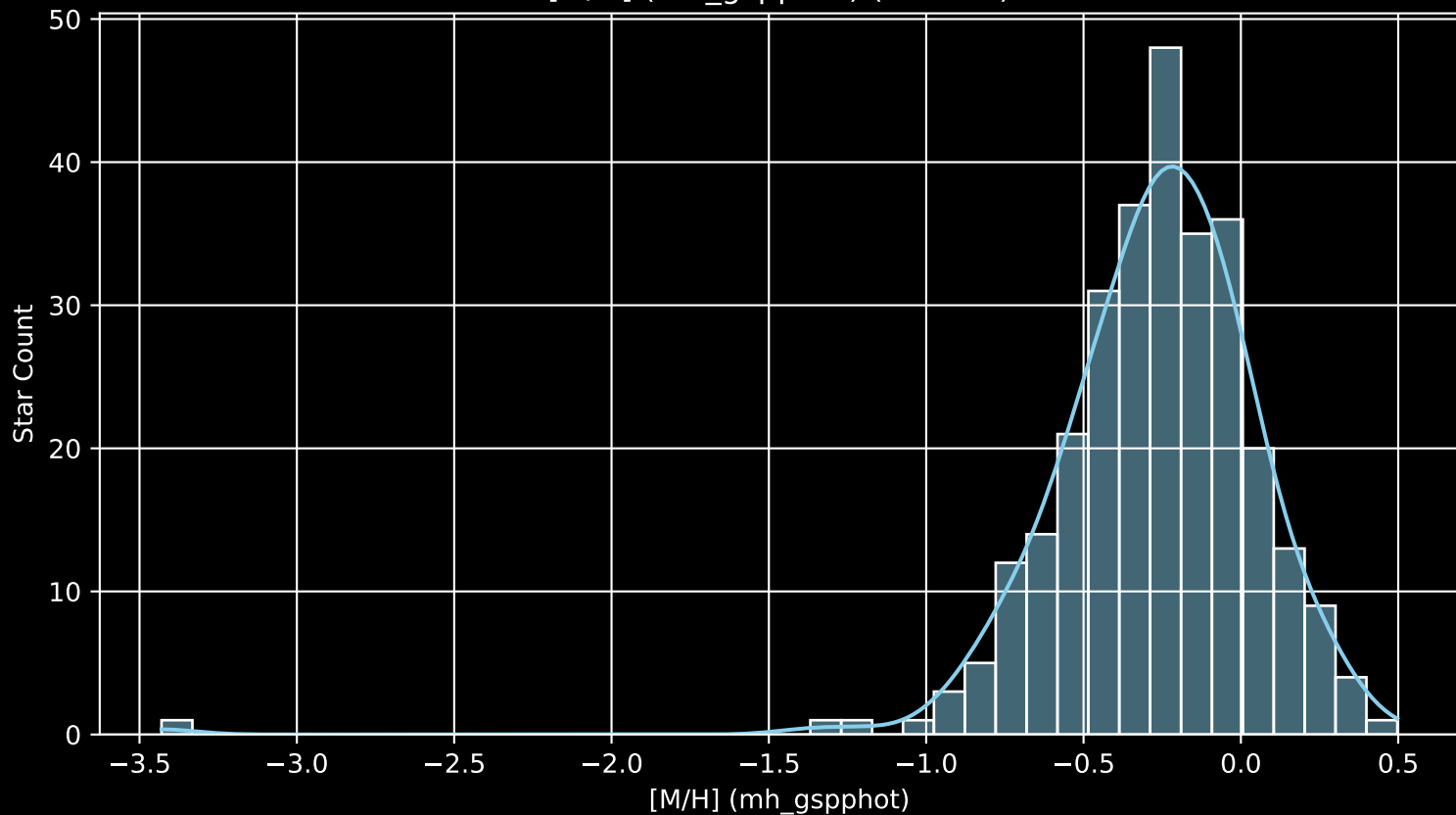
GALAH DR4 Field: [6927] [M/H] (mh_gspphot) (n= 293)
