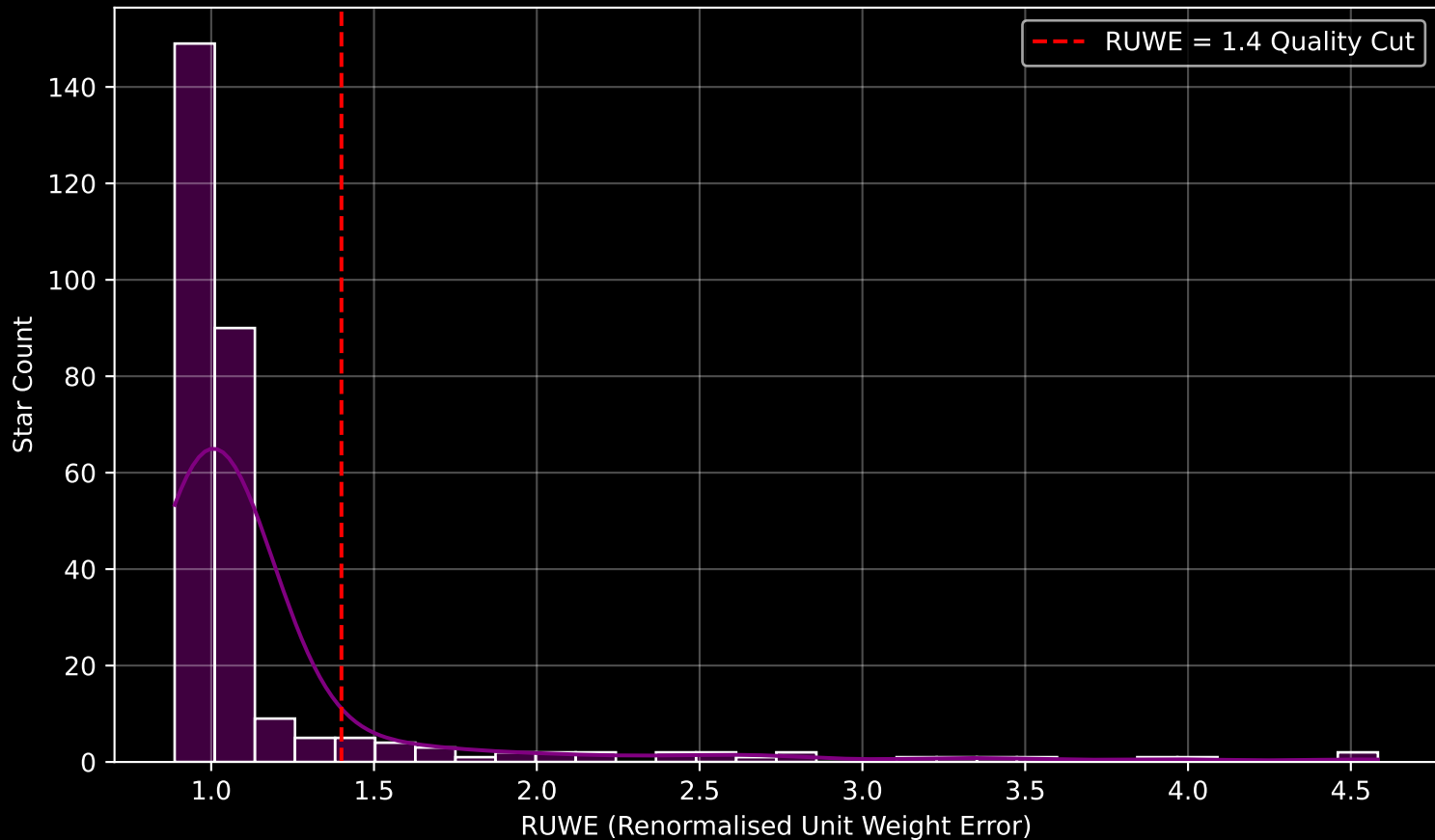
GALAH DR4 Field [6927] RUWE Distribution (n= 287)
